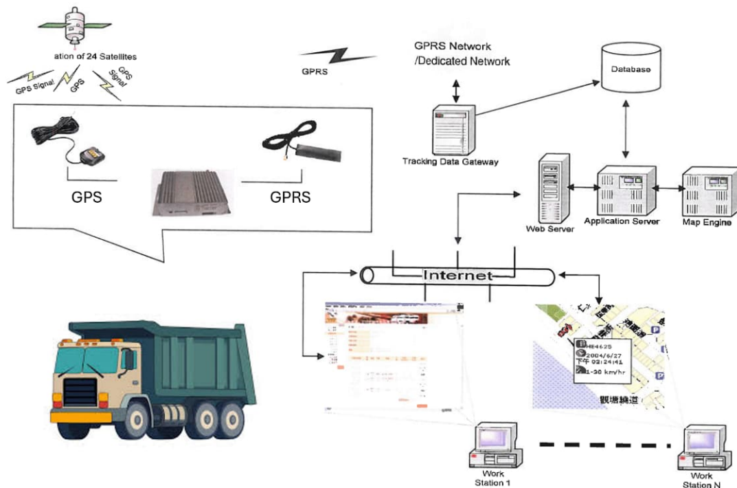
Figure 7.1 – Real time tracking system configuration
